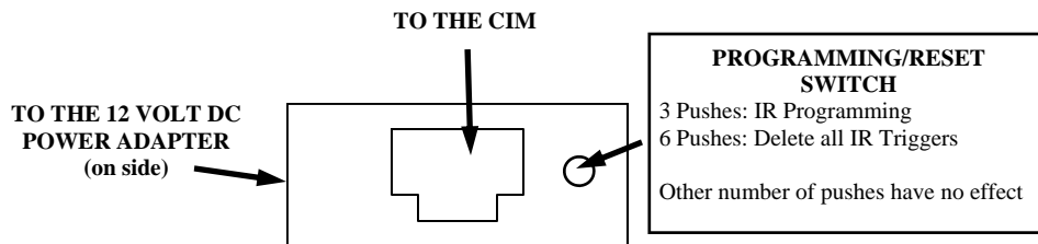
FIGURE 1: IR UPB MODULE REAR PANEL WIRE CONNECTION DIAGRAM
